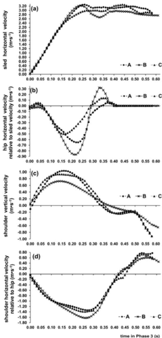
(a) sled horizontal velocity (b) hip horizontal velocity relative to the sled (c) shoulder vertical velocity (d) shoulder horizontal velocity relative to the hip Figure 2. Average velocities with respect to Phase 3 duration
